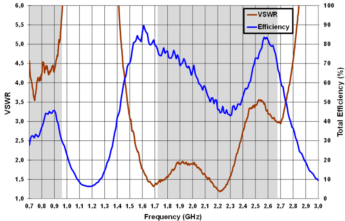
Figure 3 – VSWR and Total Efficiency for the 698 – 960 MHz frequency range and for the 1710 – 2690 MHz frequency range (from the evaluation board (Figure 1)).
