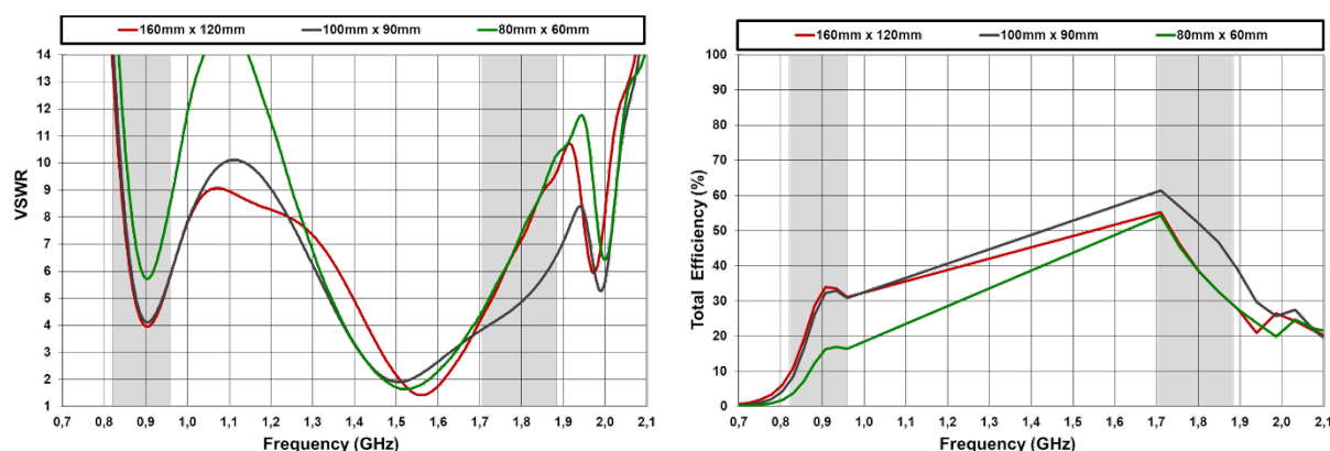
Figure 8 – Comparison VSWR and antenna efficiency for different PCB sizes (Figure 7) considering the same matching network considered in the C1-RS module in all the platforms , from 824MHz to 960MHz, and from 1710MHz to 1880MHz (Figure 4).
