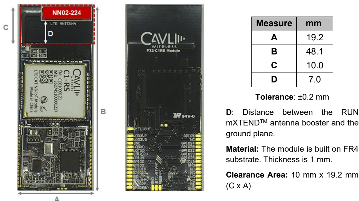
Figure 3 – P32 C1-RS Module integrates the RUN mXTEND ™ , providing operation from 824MHz to 960MHz, and from 1710MHz to 1880MHz. Top view in the left and bottom view in the right.
