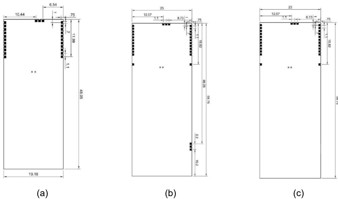
Figure 2- P32 series modules dimensions. (a) P32 C1-RS module, (b) P32 C31-QM module and (c) P32 C1-RM module.
