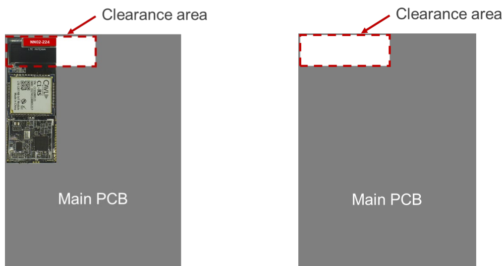
Figure 6 – On the left side, an example of the P32 C1-RS module integration in a particular device, and in the right side, an example of the main board ground plane and the required clearance area.
