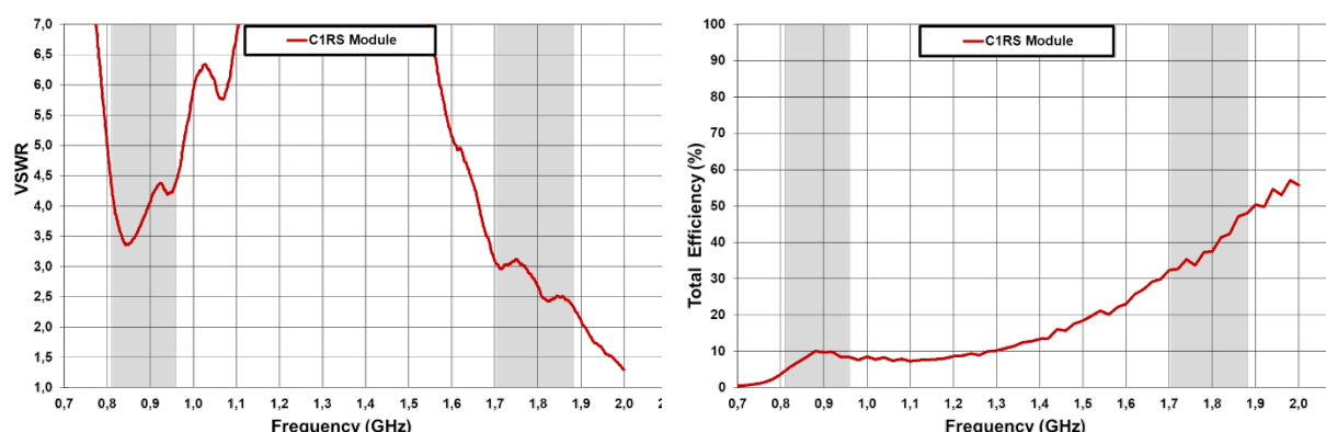
Figure 5 –VSWR and Antenna Efficiency in the C1-RS module, from 824MHz to 960MHz, and from 1710MHz to 1880MHz (Figure 4).
