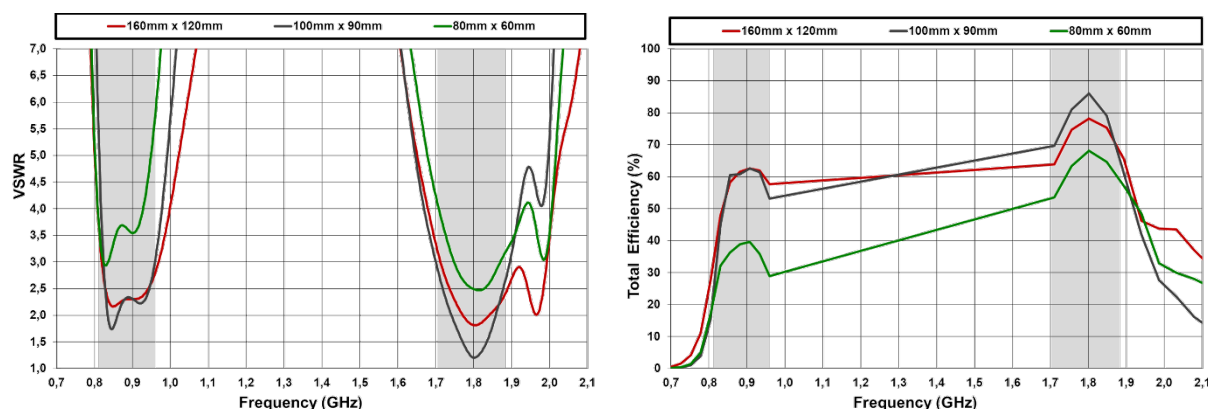
Figure 9 – Comparison VSWR and Antenna Efficiency by changing the Main PCB dimensions considering the optimized matching network for each platform , for 824MHz to 960MHz, and from 1710MHz to 1880MHz (Figure 4).
