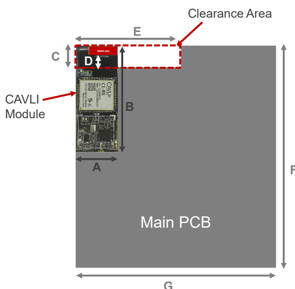
Figure 7 – P32 C1-RS module integrated in a main board for providing operation from 824MHz to 960MHz, and from 1710MHz to 1880MHz.
