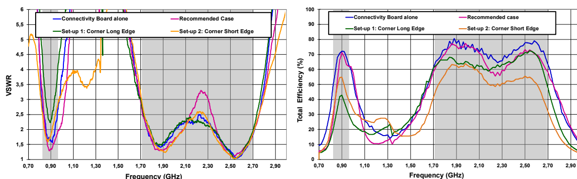
Figure 4 – VSWR and Total Efficiency for the 824 – 960 MHz frequency range and for the 1710 – 2690 MHz frequency range (the connectivity board alone; the connectivity board connected to the main board for the recommended case and two other scenarios).
